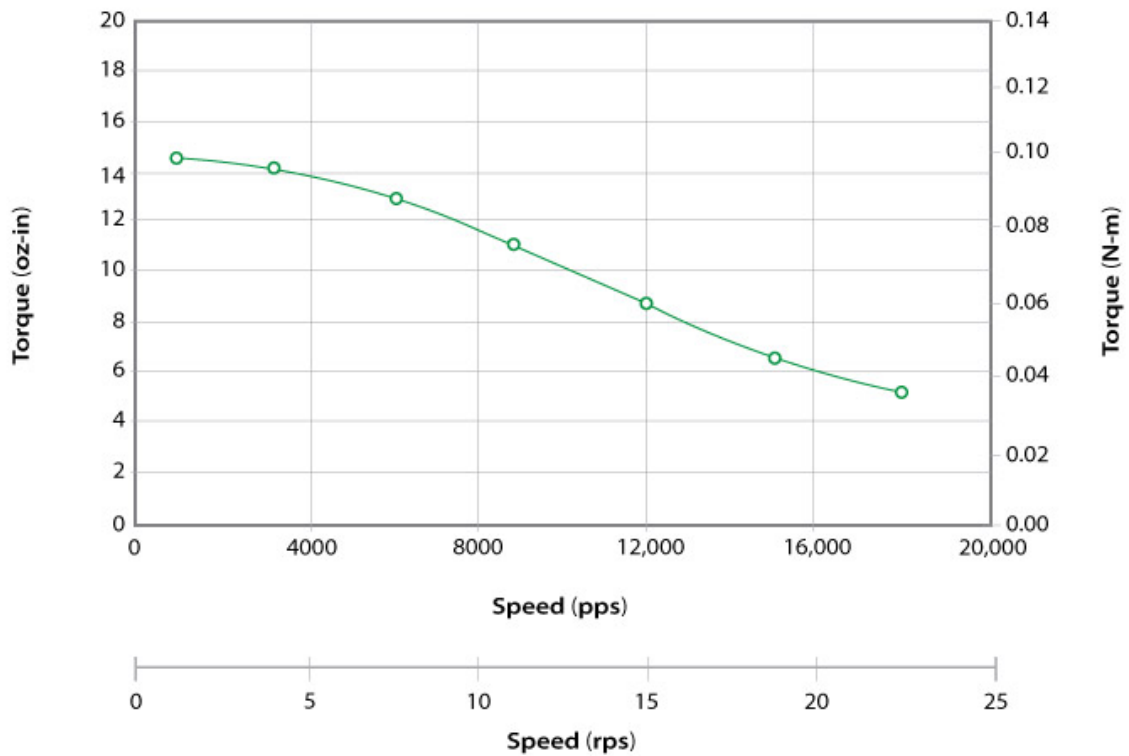
3809V-03 24VDC, 1.2 Amps/Phase, Bipolar, 1/2 Stepping
